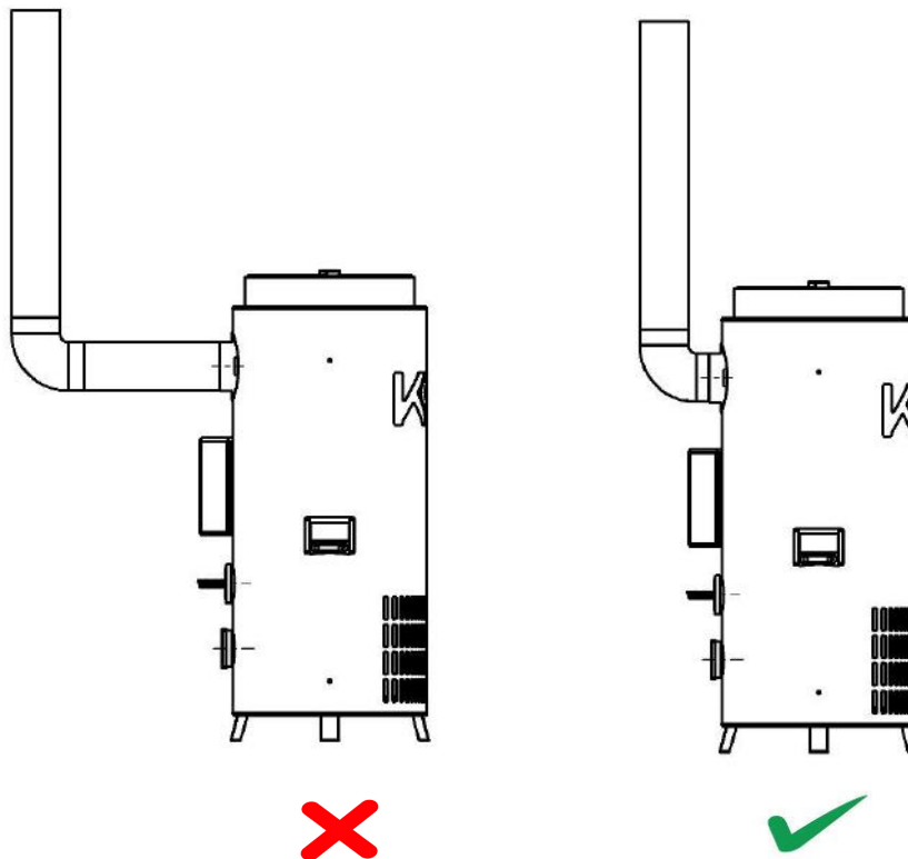
Figure4: Flue Installation
